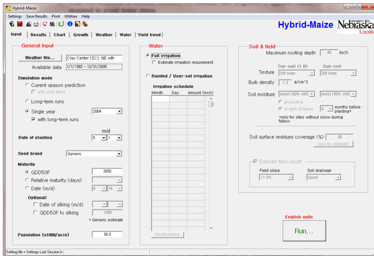
Figure 2.1: Hybrid-maize model along with inputs.
