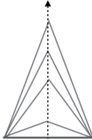
Figure 3.1: Different triangles with same base and different heights
