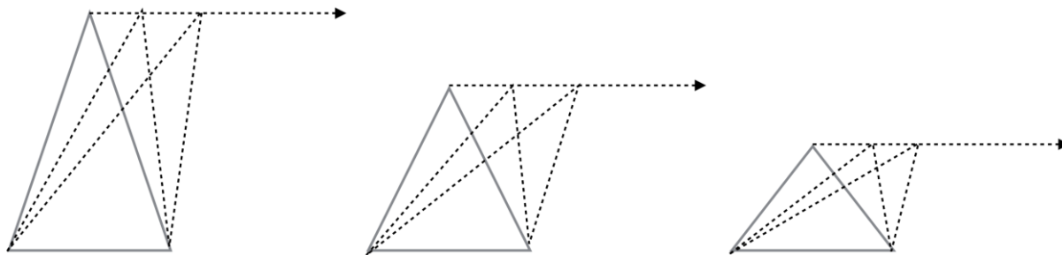
Figure 3.3: Sliding three triangles with same base and different height horizontally
